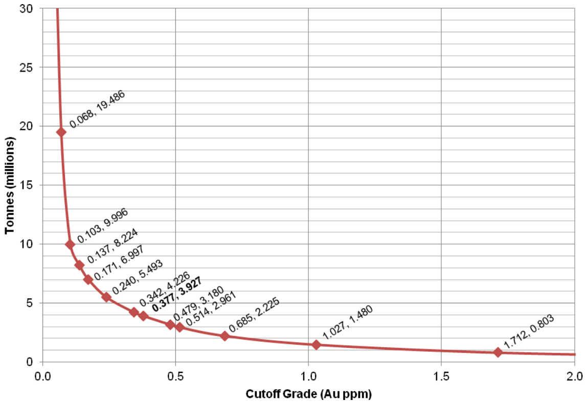
Figure 14.10 – Metric Grade-Tonnage Curve for Measured and Indicated Gold Resources
