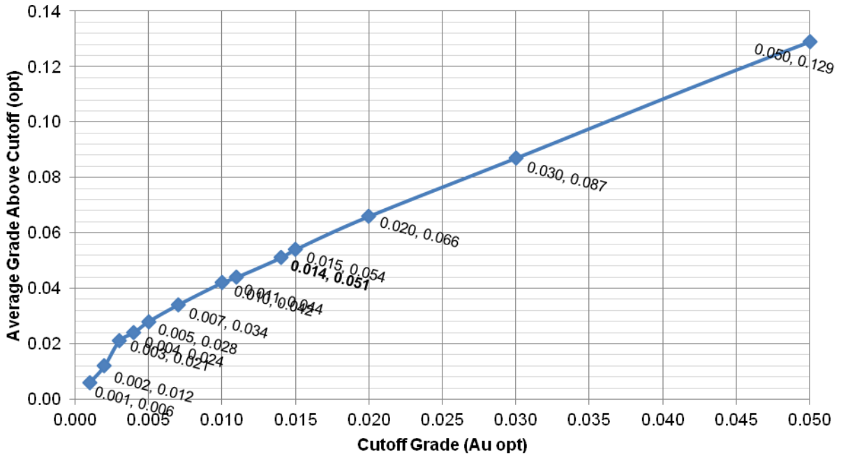
Figure 14.11 – Imperial Cutoff Grade vs. Average Grade Above Cutoff for Measured and Indicated Gold Resources
