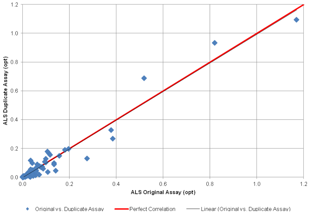
Figure 12.6A – Wilson Deposit Duplicate Assays (All Samples)
