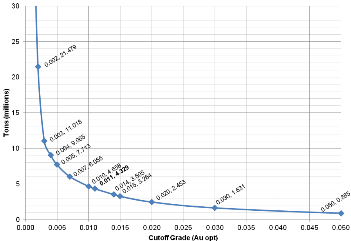
Figure 14.9 – Imperial Grade-Tonnage Curve for Measured and Indicated Gold Resources
