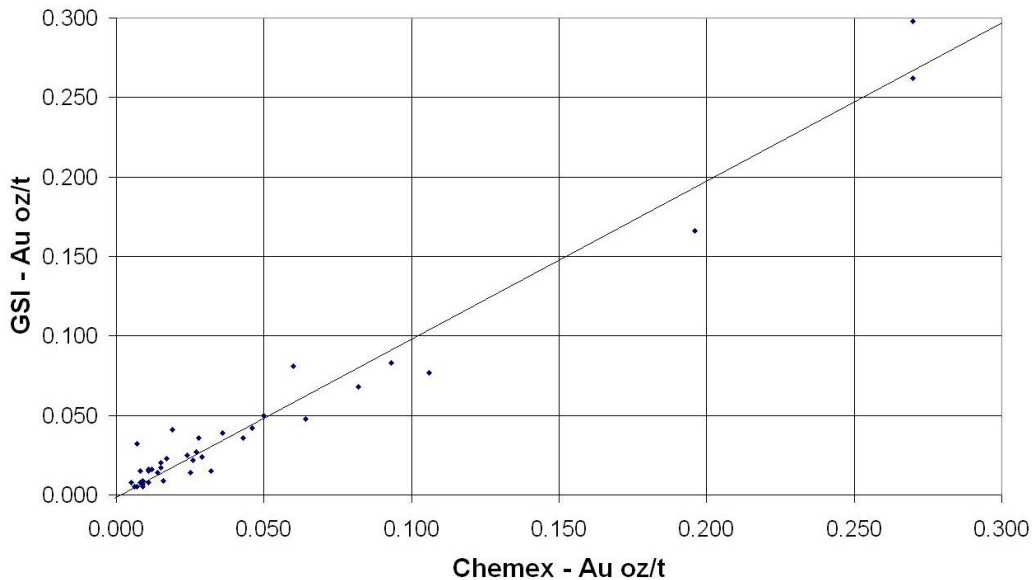
Figure 12.1 – UG Pulp Check Assays – Chem vs. GSI >0.005
