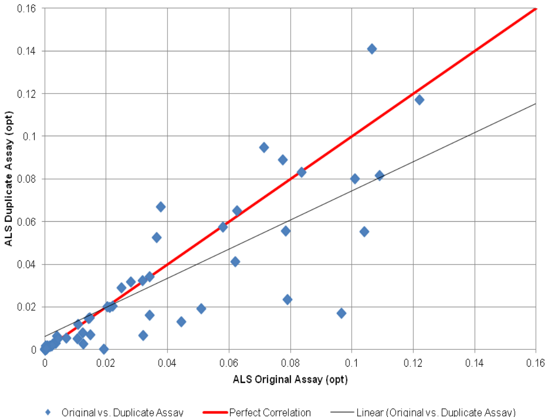
Figure 12.6D – Wilson Deposit Duplicate Assays (Samples < 0.16 opt)
