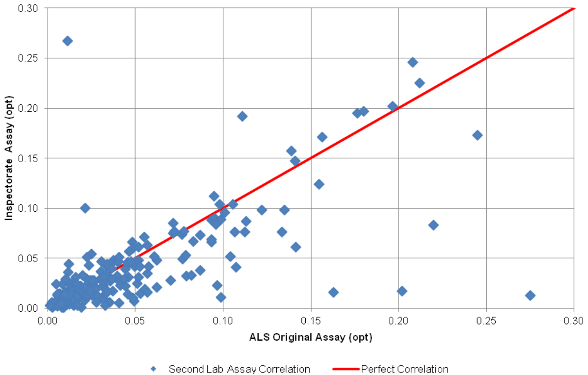
Figure 12.7B – Second Laboratory Assay Comparison (<0.3 opt)
