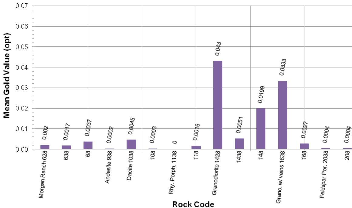
Figure 14.6 – Mean Gold Value by Rock Code in Faulted Rock Types with some Clay as Fault Gouge
