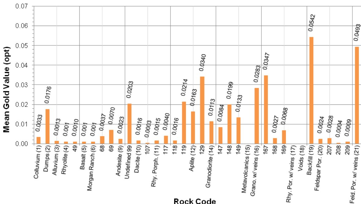
Figure 14.4 – Mean Gold Value by Rock Code in Oxide Rock Types
