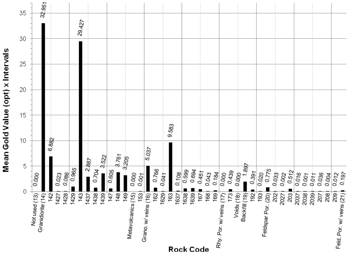
Figure 14.8B – Weighted Average of Average Gold Grade Times Number of Intervals for Rock Codes 13 Through 21
