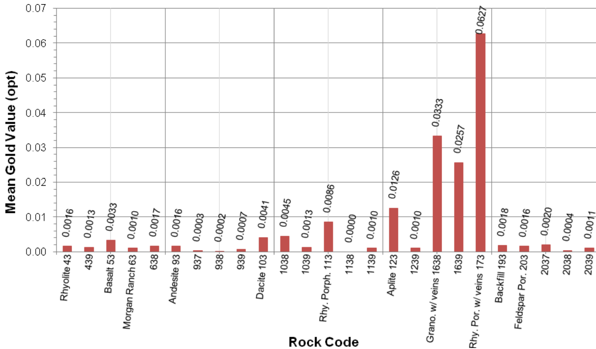
Figure 14.2 – Mean Gold Value by Rock Code in Sulfide Rock Types
