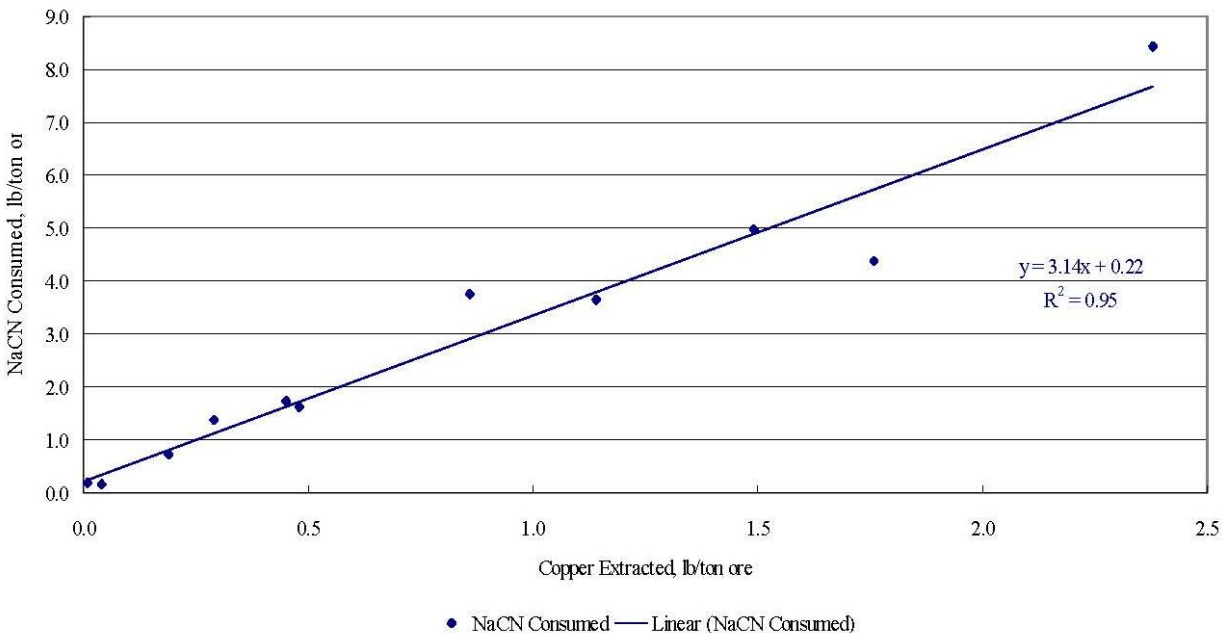
Figure 13.1 – Cyanide Consumption vs. Copper Dissolution, Bottle Roll Tests, Pine Grove Cuttings Samples, 1/4” Feeds
