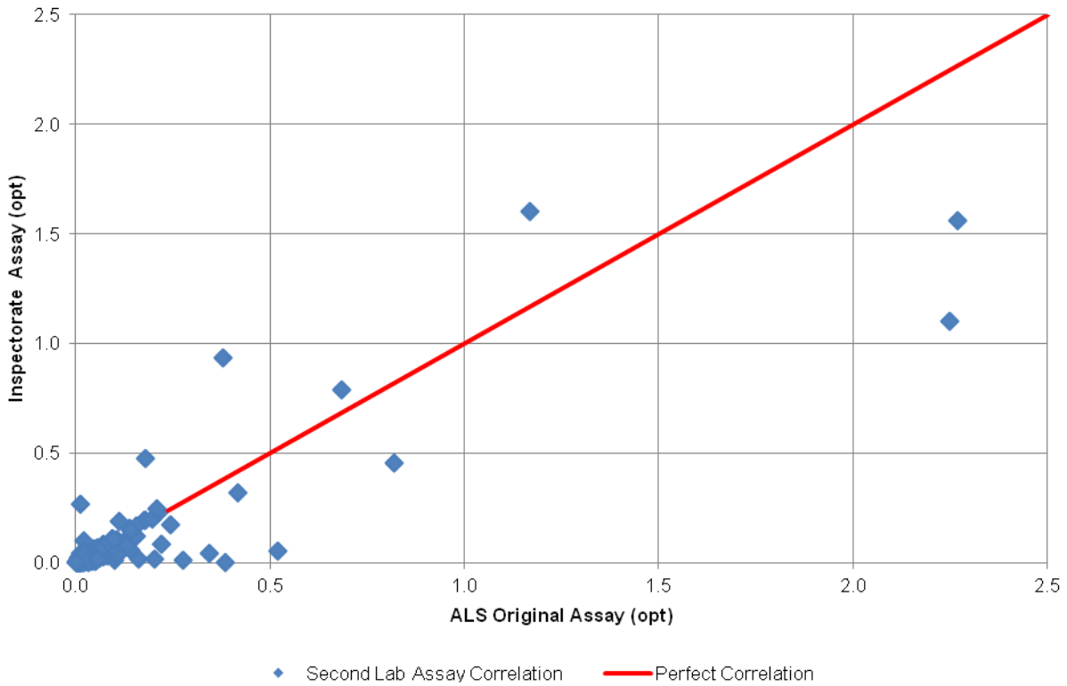
Figure 12.7A – Second Laboratory Assay Comparison
