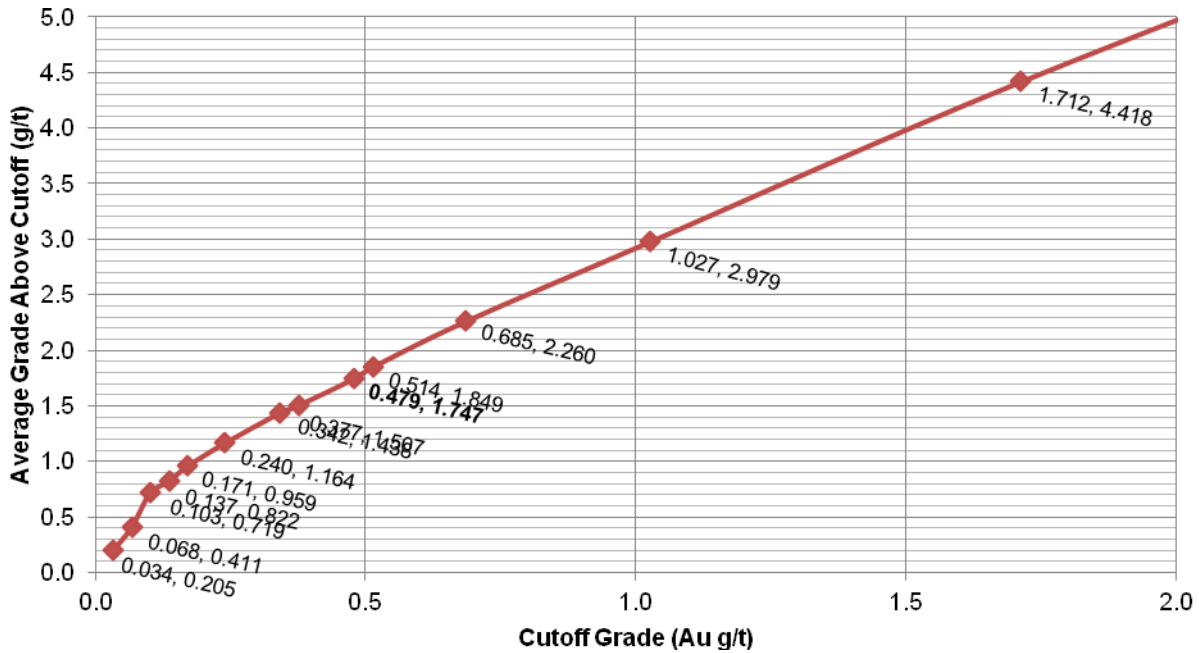
Figure 14.12 – Metric Cutoff Grade vs. Average Grade Above Cutoff for Measured and Indicated Gold Resources
