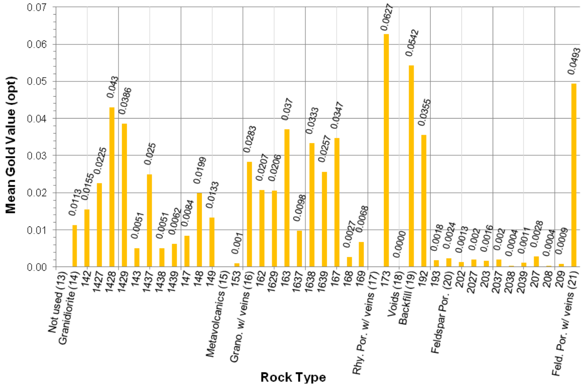
Figure 14.1B – Mean Gold Value by Rock Code in Drillhole Assays
