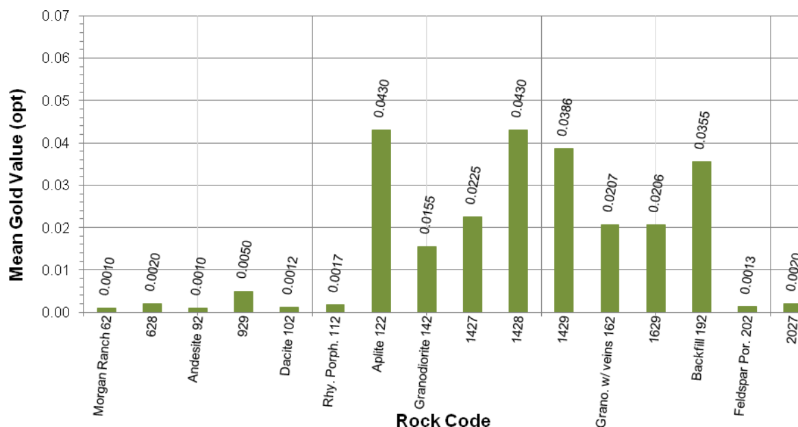
Figure 14.3 – Mean Gold Value by Rock Code in Mixed Oxide and Sulfide Rock Types
