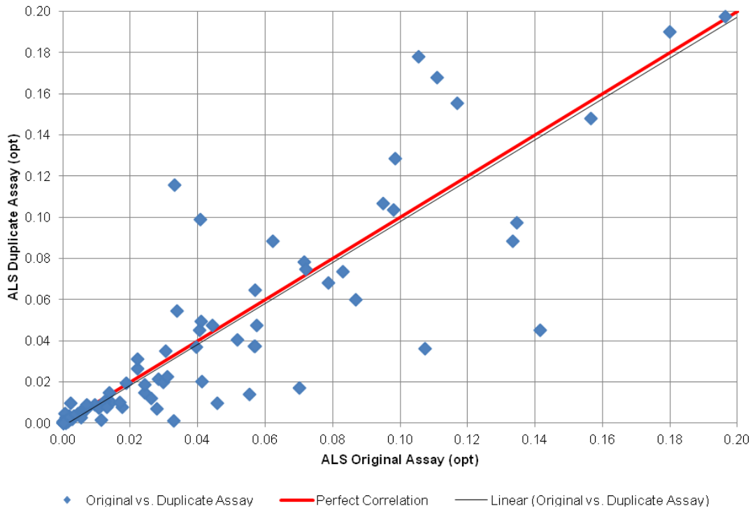
Figure 12.6B – Wilson Deposit Duplicate Assays (Samples < 0.2 opt)
