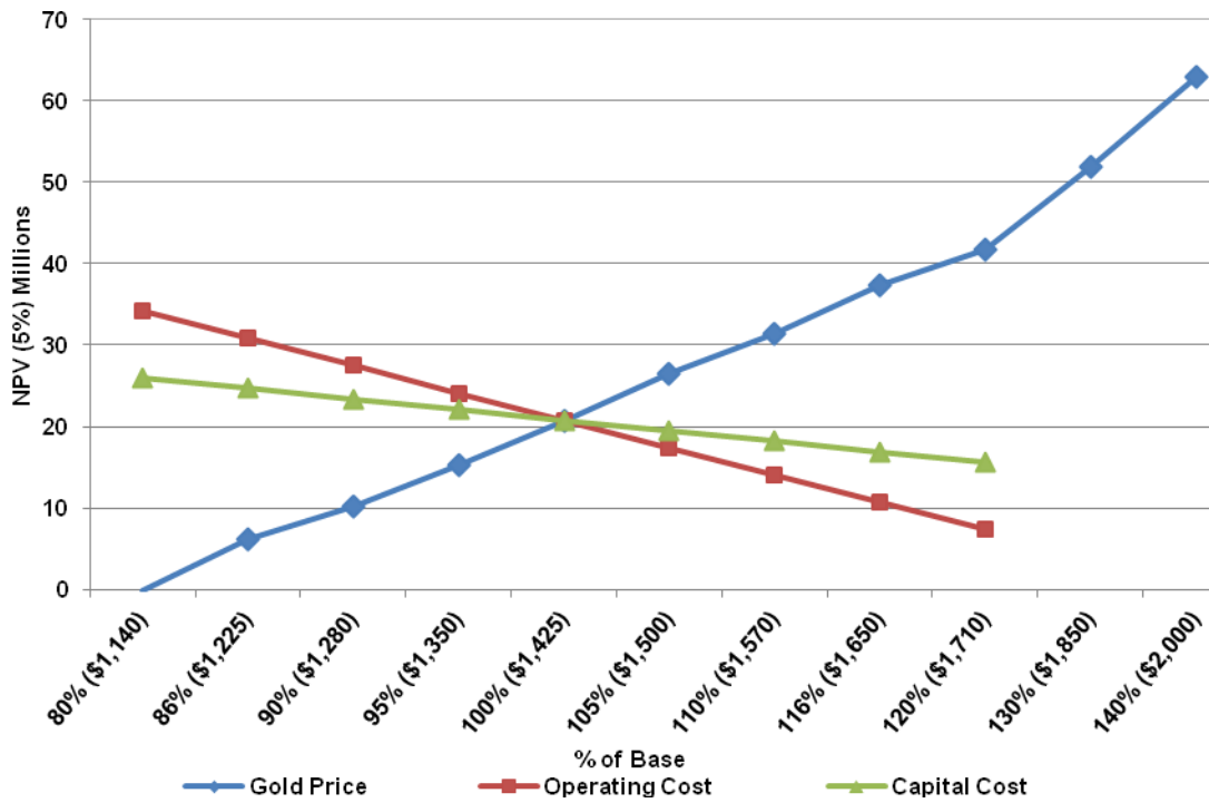
Figure 22.1 – Pine Grove Project Sensitivity (NPV 5%)
