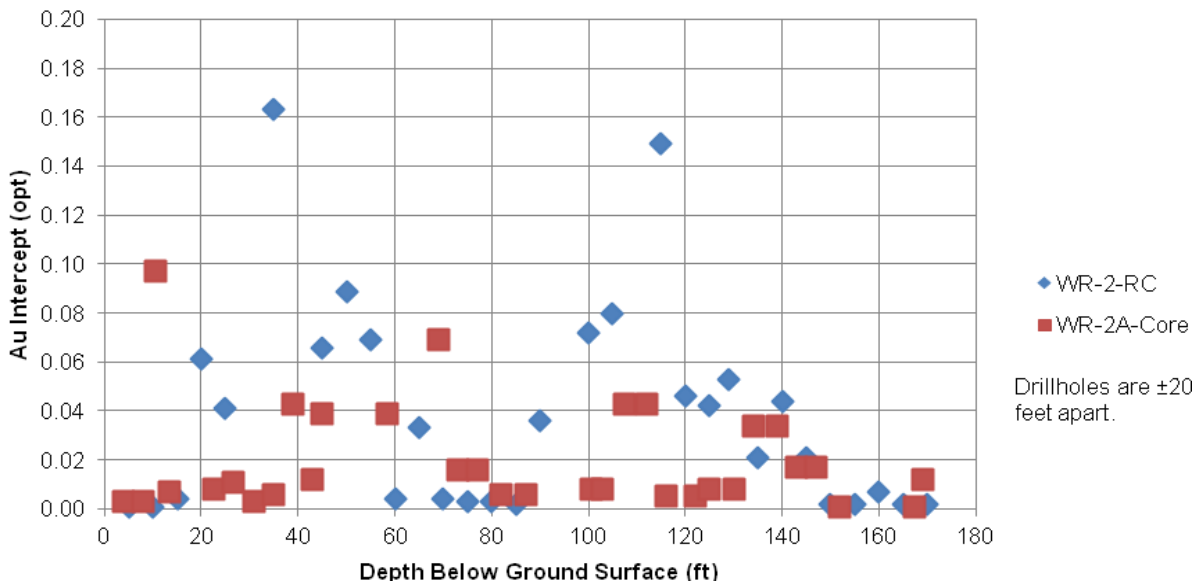
Figure 12.11A – WR-2 (RC) vs. WR-2A (Core) Comparison
