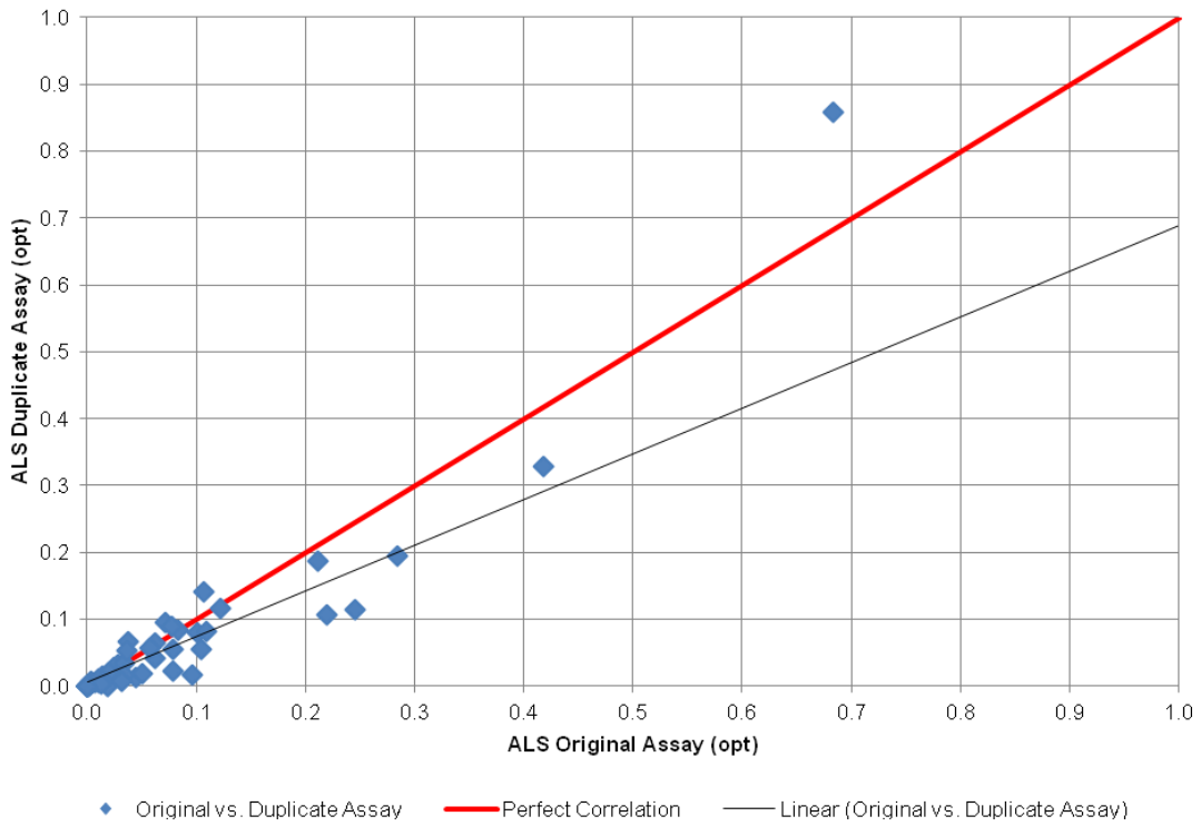
Figure 12.6C – Wheeler Deposit Duplicate Assays (All Samples)
