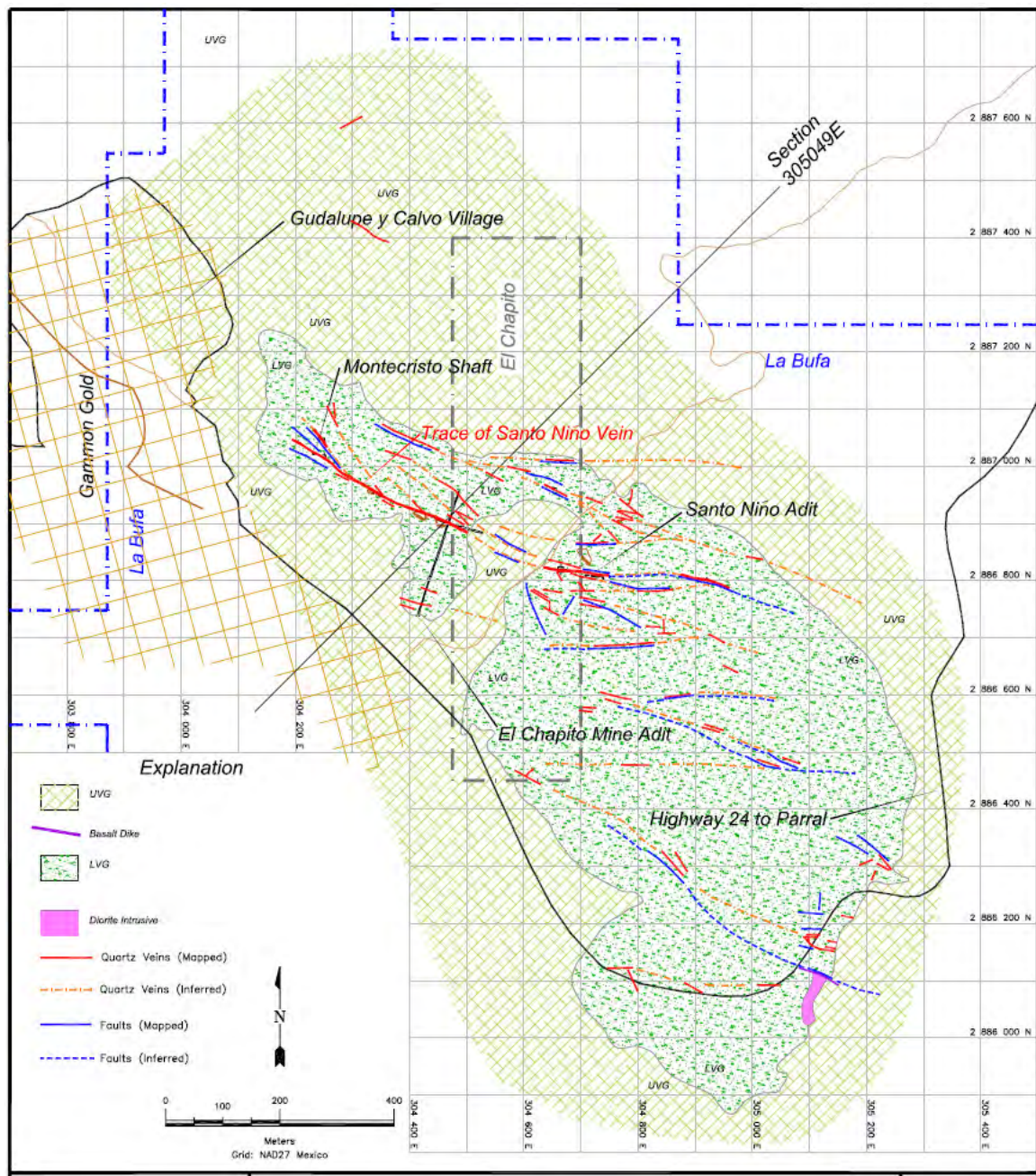
Figure 9.3 Interpretive Geology and Vein Structure Map Geology Compiled and Modified from: 1.) Bybee, 2007, La Bufa Concession Southern Area Geology Map
