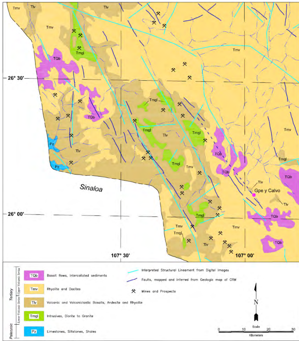
Figure 9.1 Regional Geology
