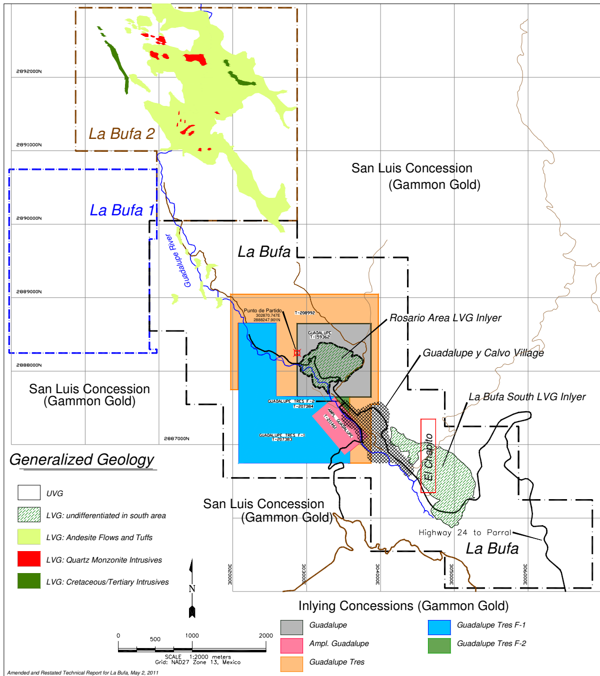
Figure 9.2 Generalized Geology Guadalupe District
